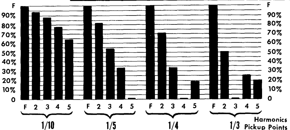
PERCENTAGE DISTRIBUTION OF HARMONICS AT THE PICKUP POINTS
